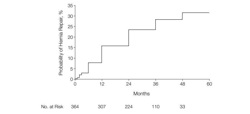
Figure 4. Probability of Crossover From Watchful Waiting to Surgery
